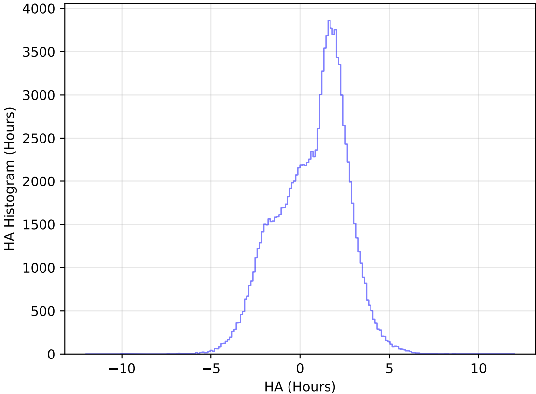
ddf_loaded_half_fl1_v3.4_10yrs All sky u band: HA Histogram
