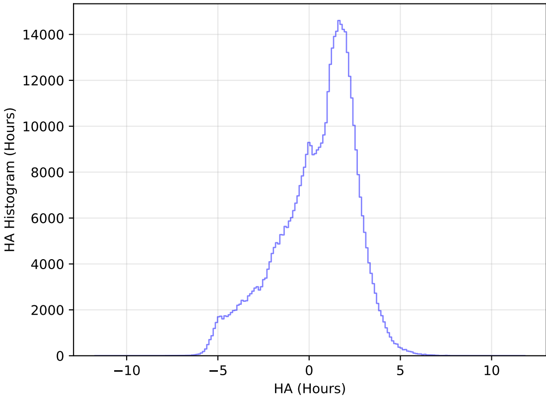
ddf_loaded_half_fl1_v3.4_10yrs All sky r band: HA Histogram
