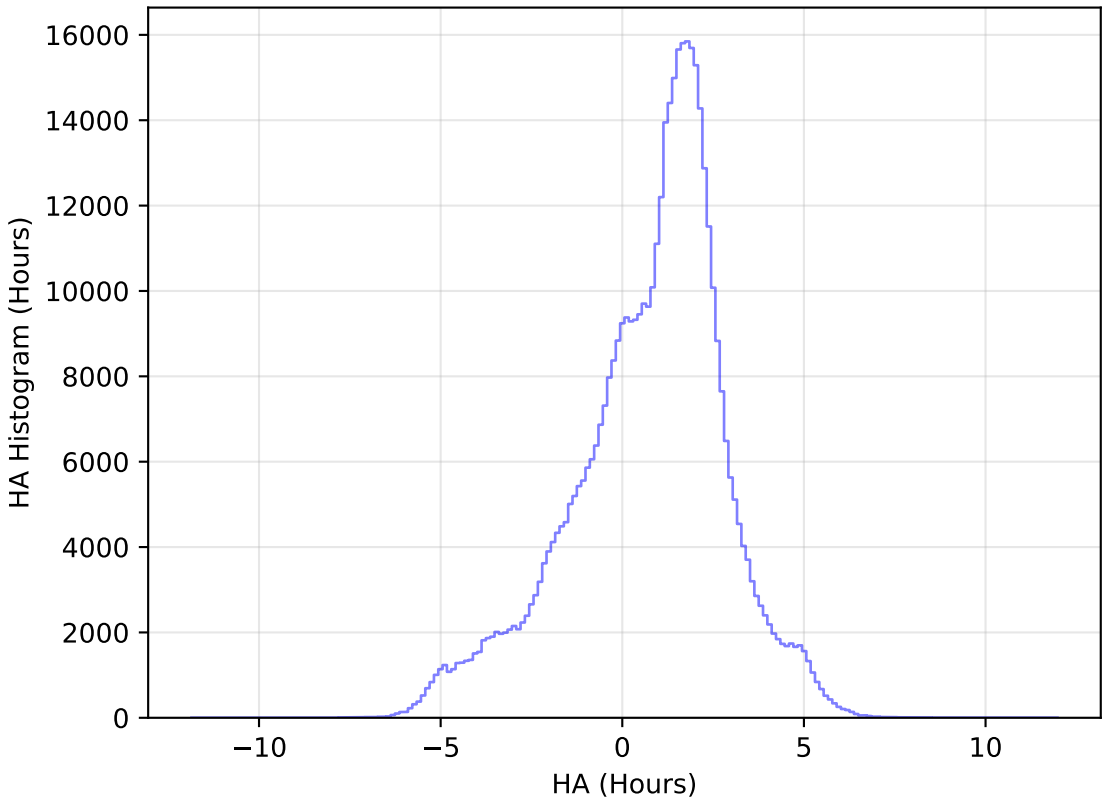
ddf_loaded_half_fl1_v3.4_10yrs All sky i band: HA Histogram
