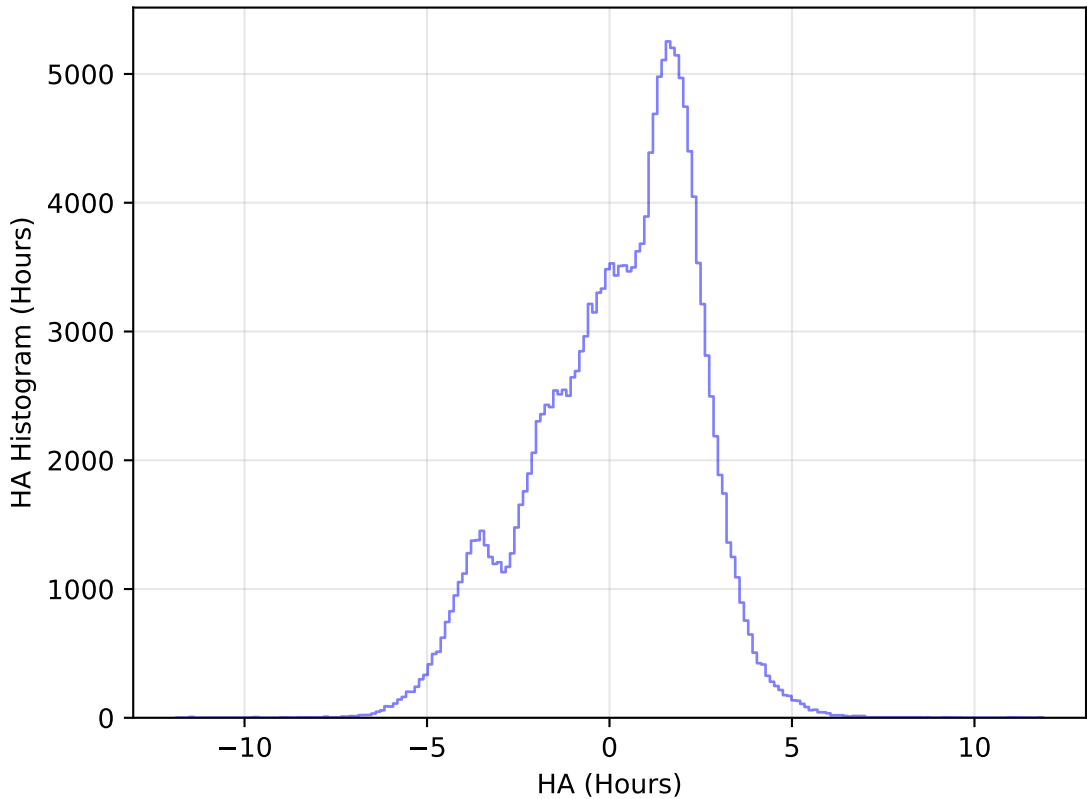
ddf_loaded_half_fl1_v3.4_10yrs All sky g band: HA Histogram
