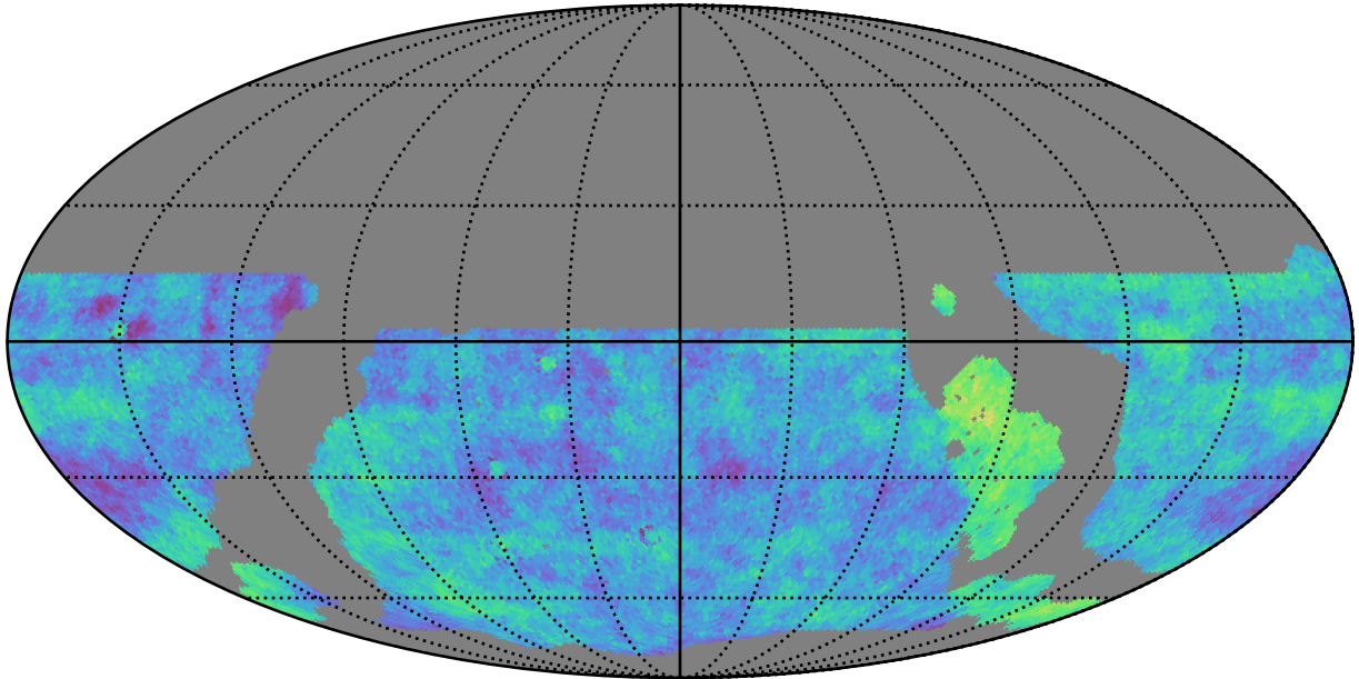
ddf_loaded_half_fl1_v3.4_10yrs gri WFD: Fraction of visits in pairs (20-90 min)
