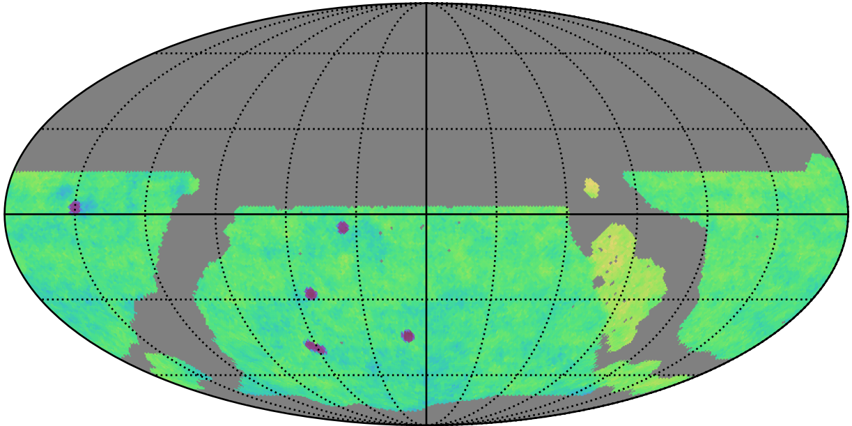
ddf_loaded_half_fl1_v3.4_10yrs gri WFD: Fraction of visits in pairs (10-60 min)
