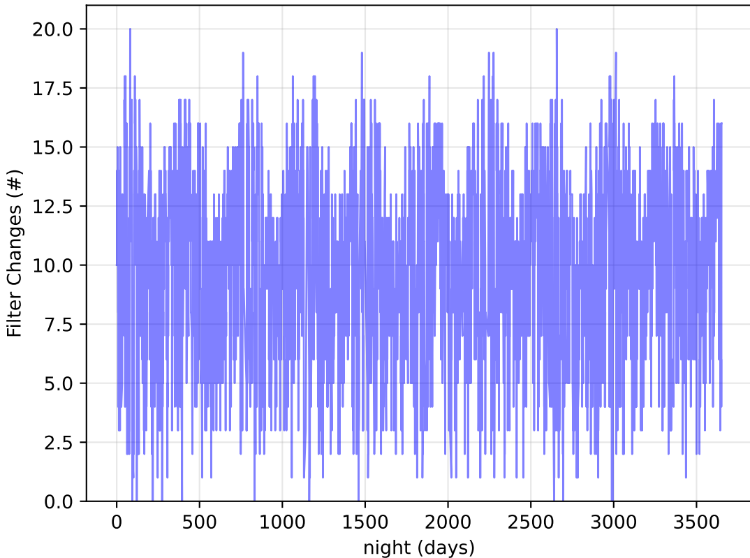
ddf_loaded_half_fl1_v3.4_10yrs Per Night: Filter Changes
