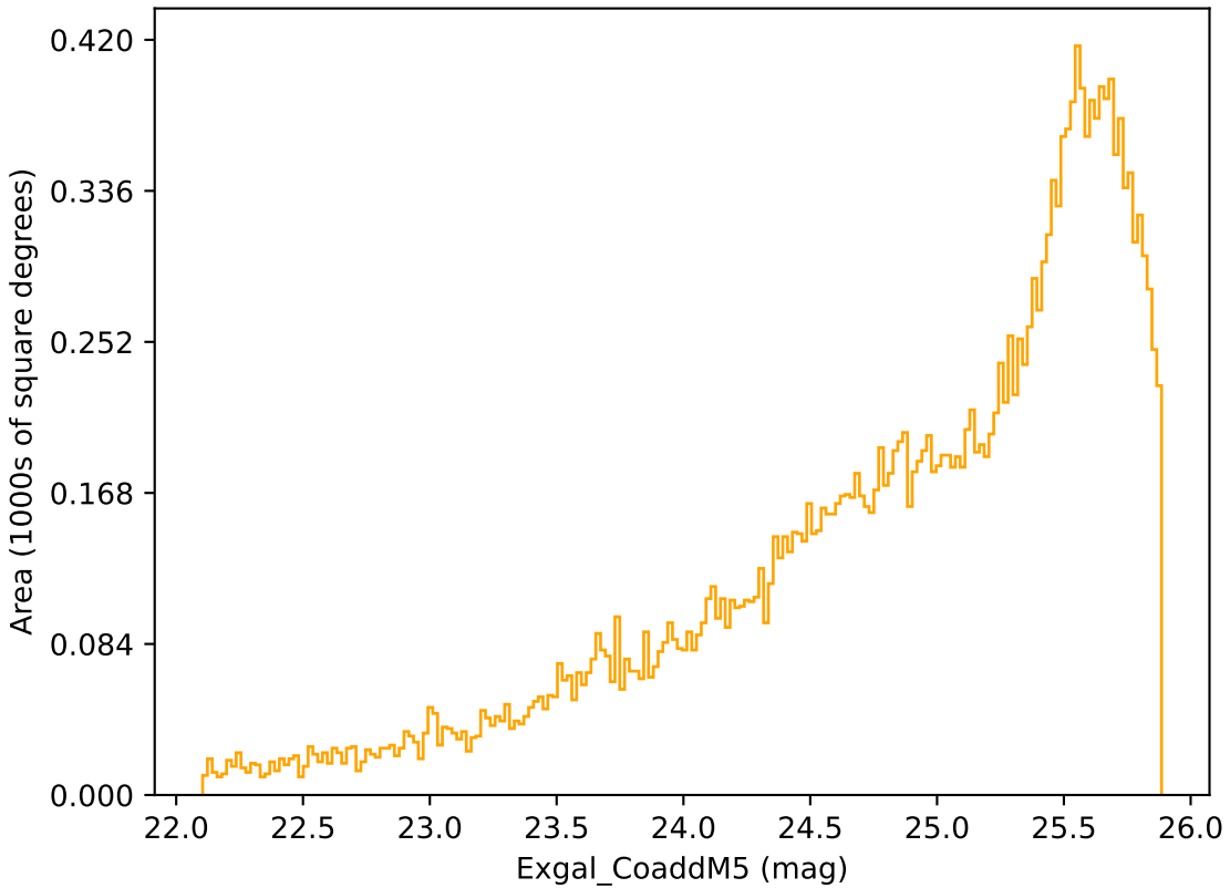
ddf_loaded_half_fl1_v3.4_10yrs Yr 3-4 r band: Exgal_CoaddM5
