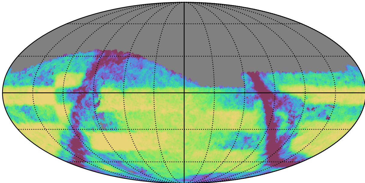
ddf_loaded_half_fl1_v3.4_10yrs Yr 3-4 i band: Exgal_CoaddM5
