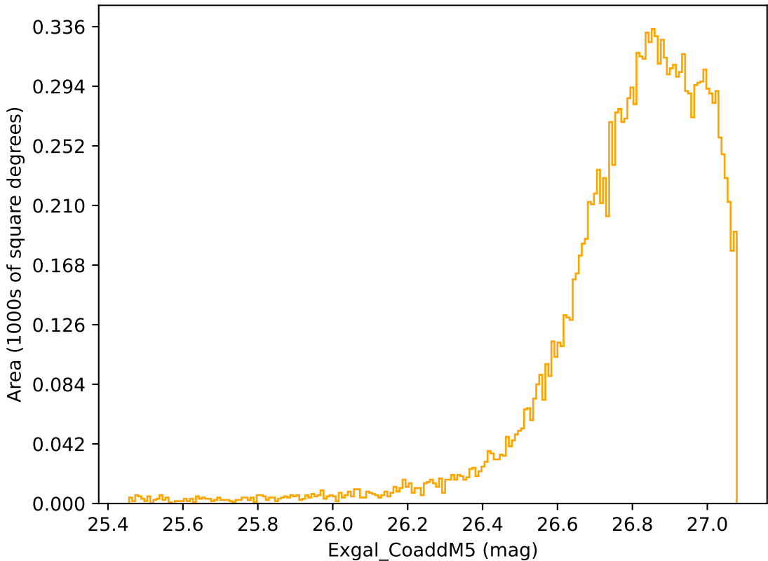
ddf_loaded_half_fl1_v3.4_10yrs WFD r band: Exgal_CoaddM5
