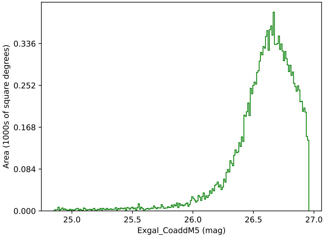
ddf_loaded_half_fl1_v3.4_10yrs WFD g band: Exgal_CoaddM5
