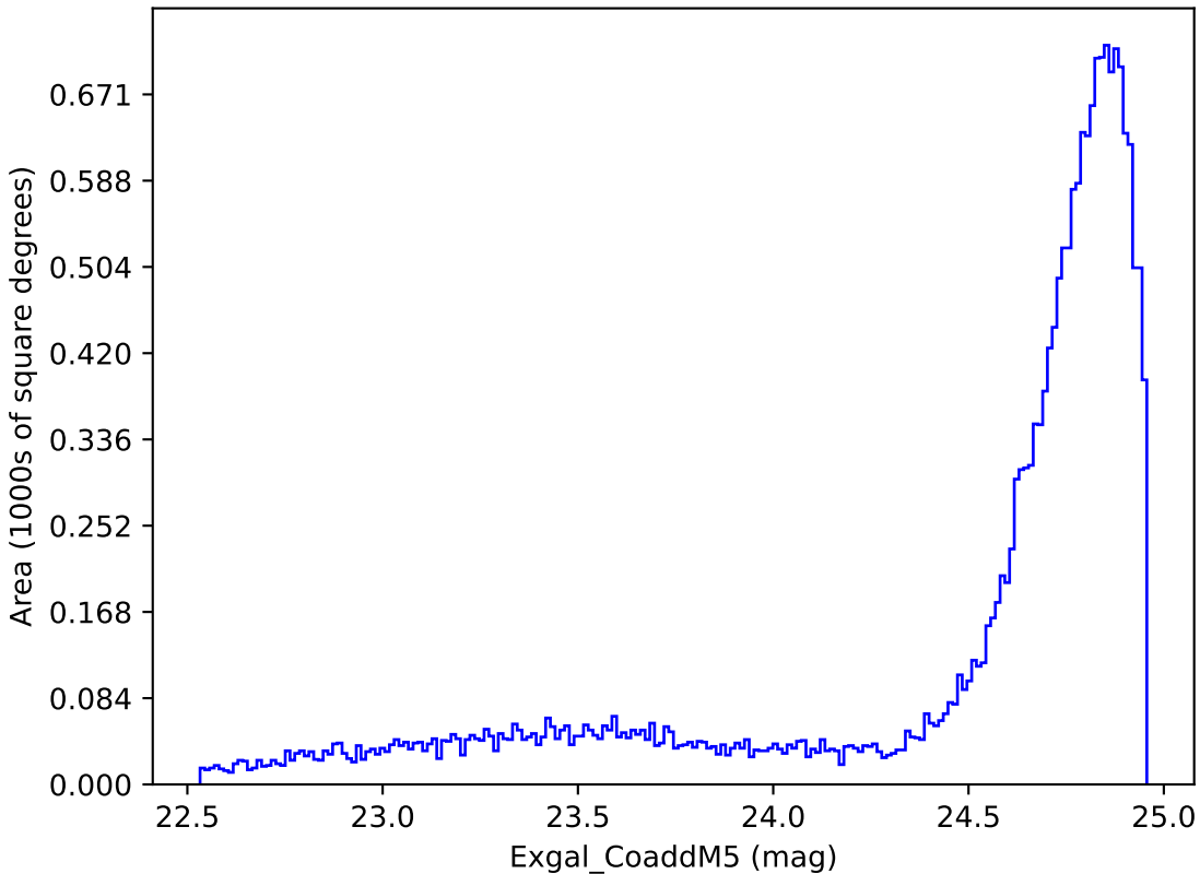
ddf_loaded_half_fl1_v3.4_10yrs All sky y band: Exgal_CoaddM5
