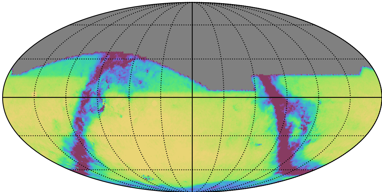
ddf_loaded_half_fl1_v3.4_10yrs All sky r band: Exgal_CoaddM5
