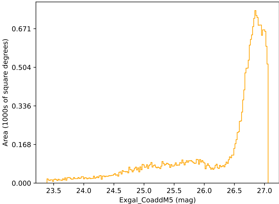
ddf_loaded_half_fl1_v3.4_10yrs All sky r band: Exgal_CoaddM5
