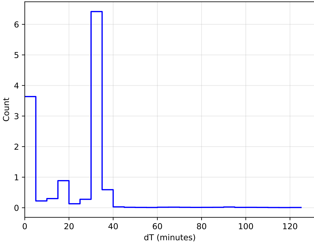
ddf_loaded_half_fl1_v3.4_10yrs All sky: DeltaT Histogram
