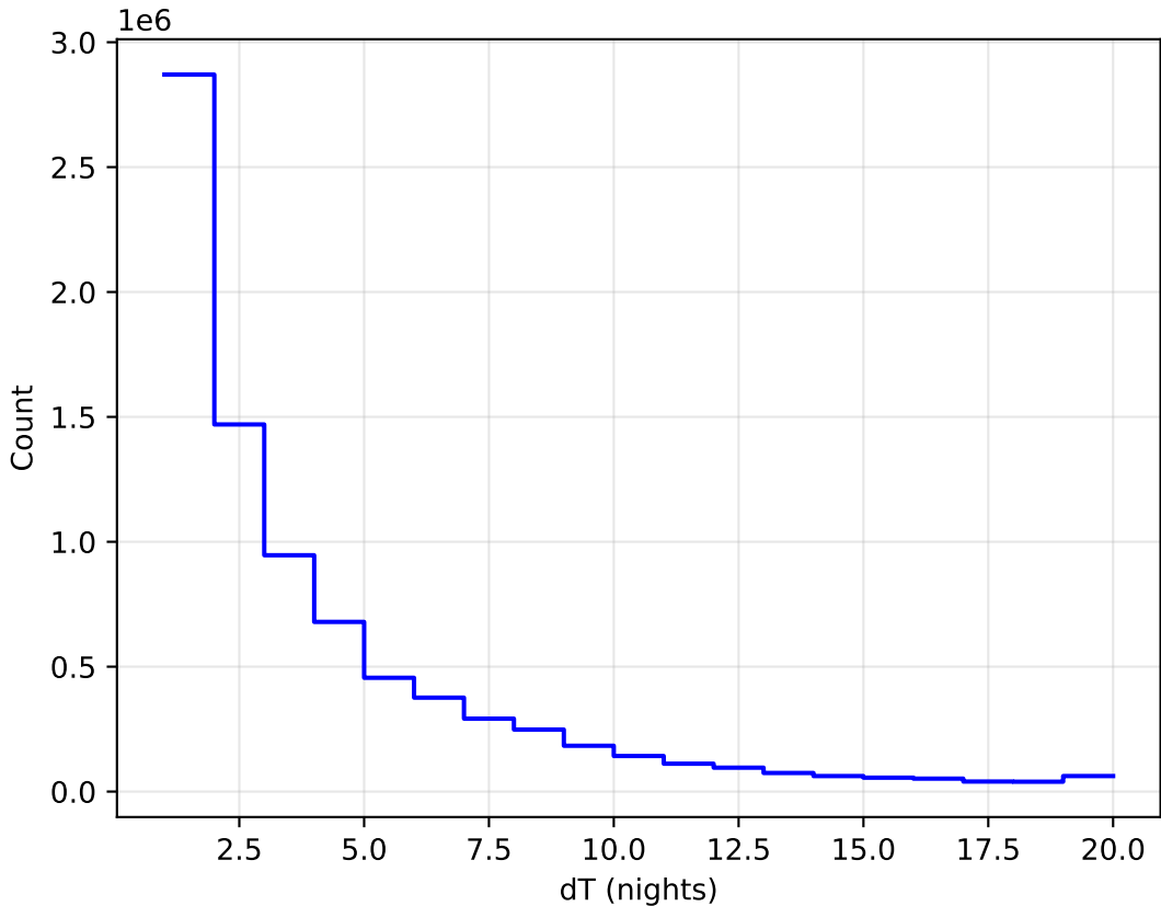
ddf_loaded_half_fl1_v3.4_10yrs WFD all bands: DeltaNight Histogram
