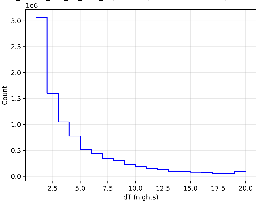
ddf_loaded_half_fl1_v3.4_10yrs All sky all bands: DeltaNight Histogram
