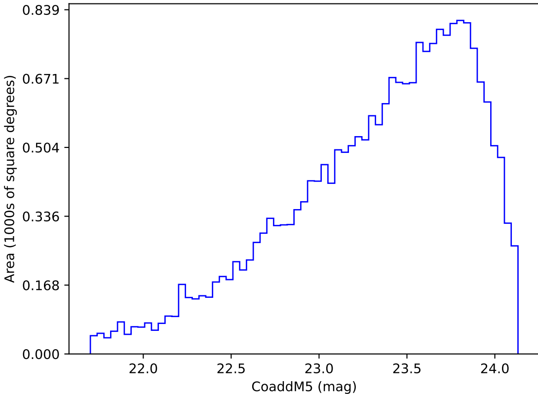
ddf_loaded_half_fl1_v3.4_10yrs Yr 3-4 y band: CoaddM5
