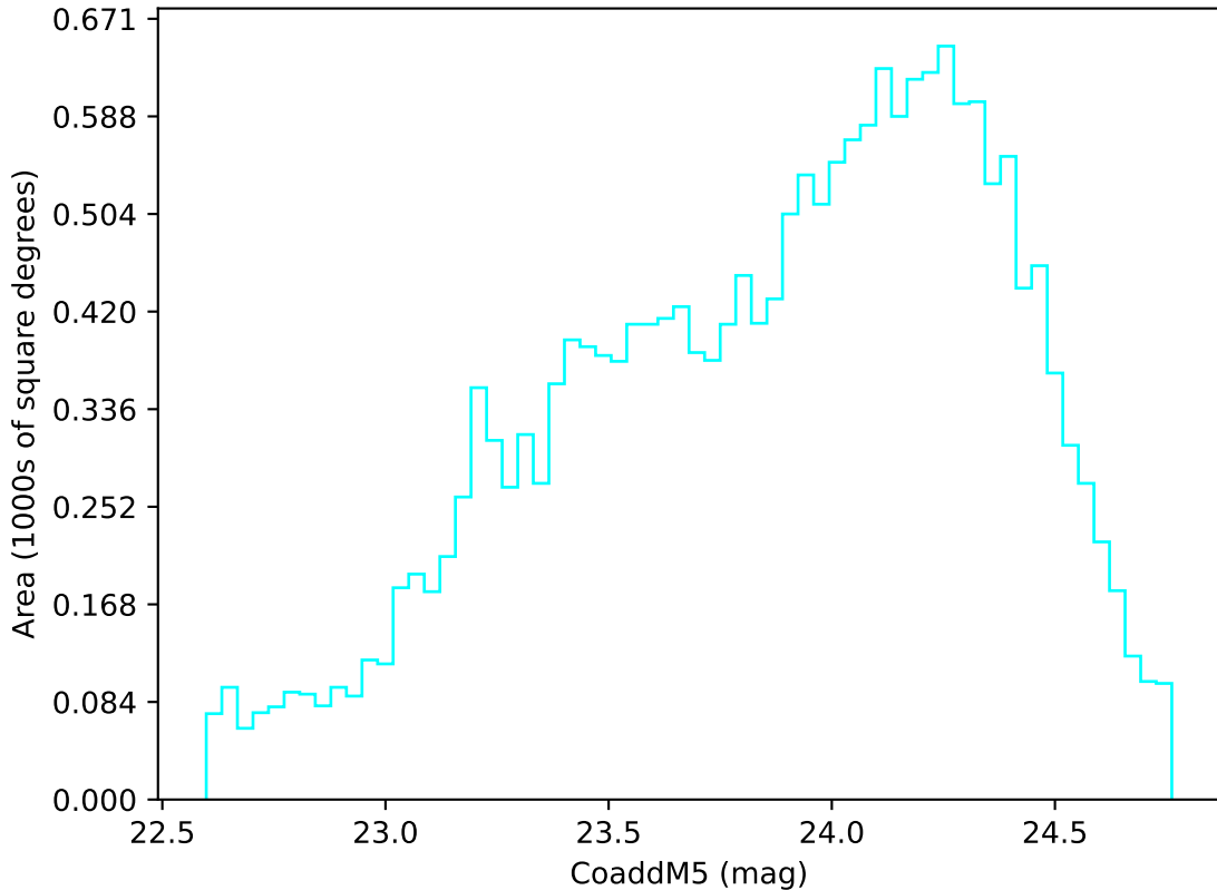
ddf_loaded_half_fl1_v3.4_10yrs Yr 3-4 u band: CoaddM5
