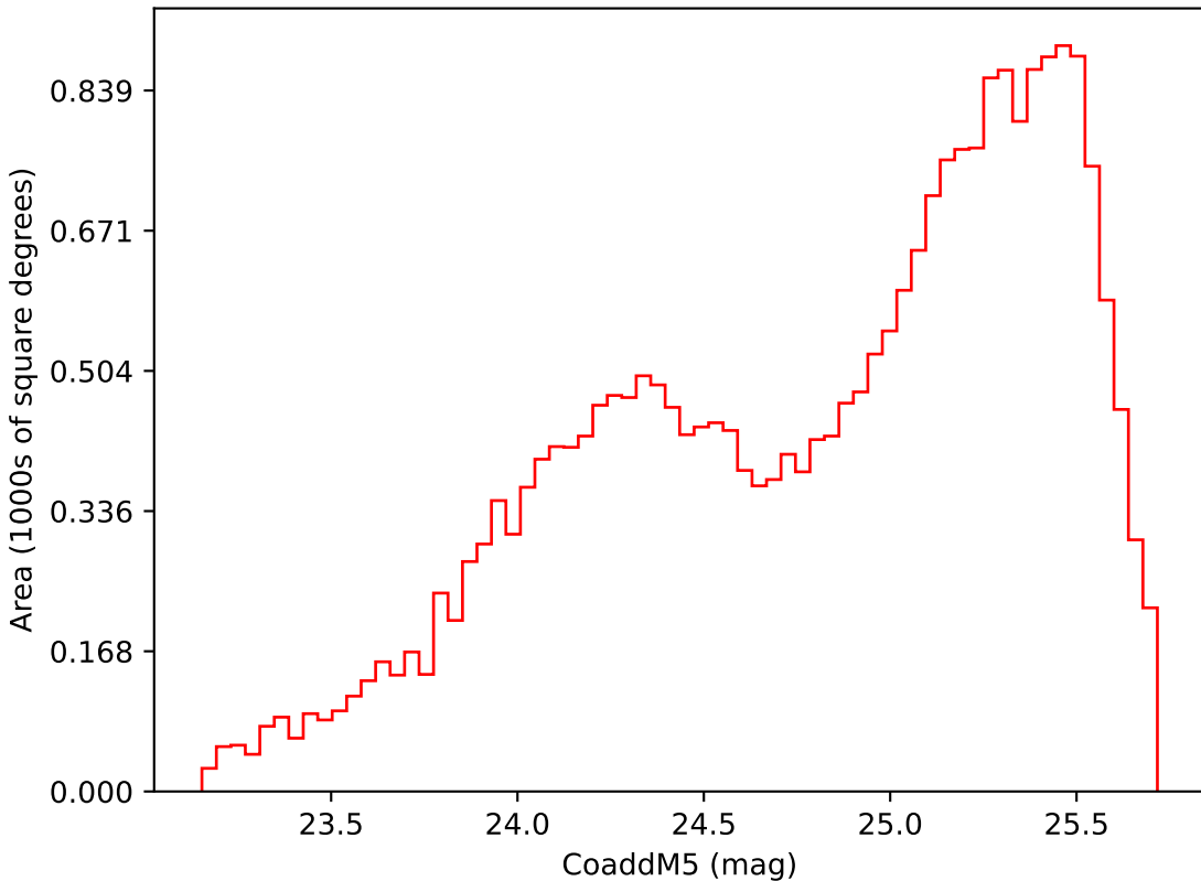
ddf_loaded_half_fl1_v3.4_10yrs Yr 3-4 i band: CoaddM5
