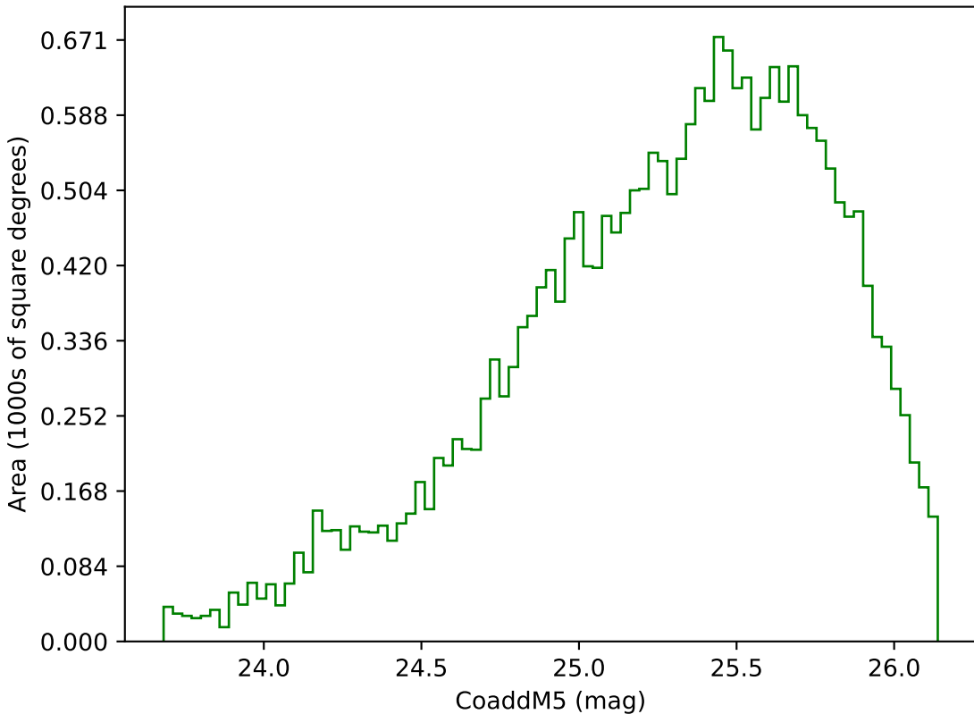
ddf_loaded_half_fl1_v3.4_10yrs Yr 3-4 g band: CoaddM5
