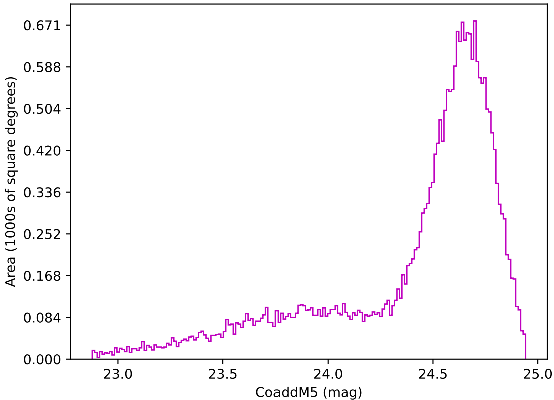
ddf_loaded_half_fl1_v3.4_10yrs Yr 1 z band: CoaddM5
