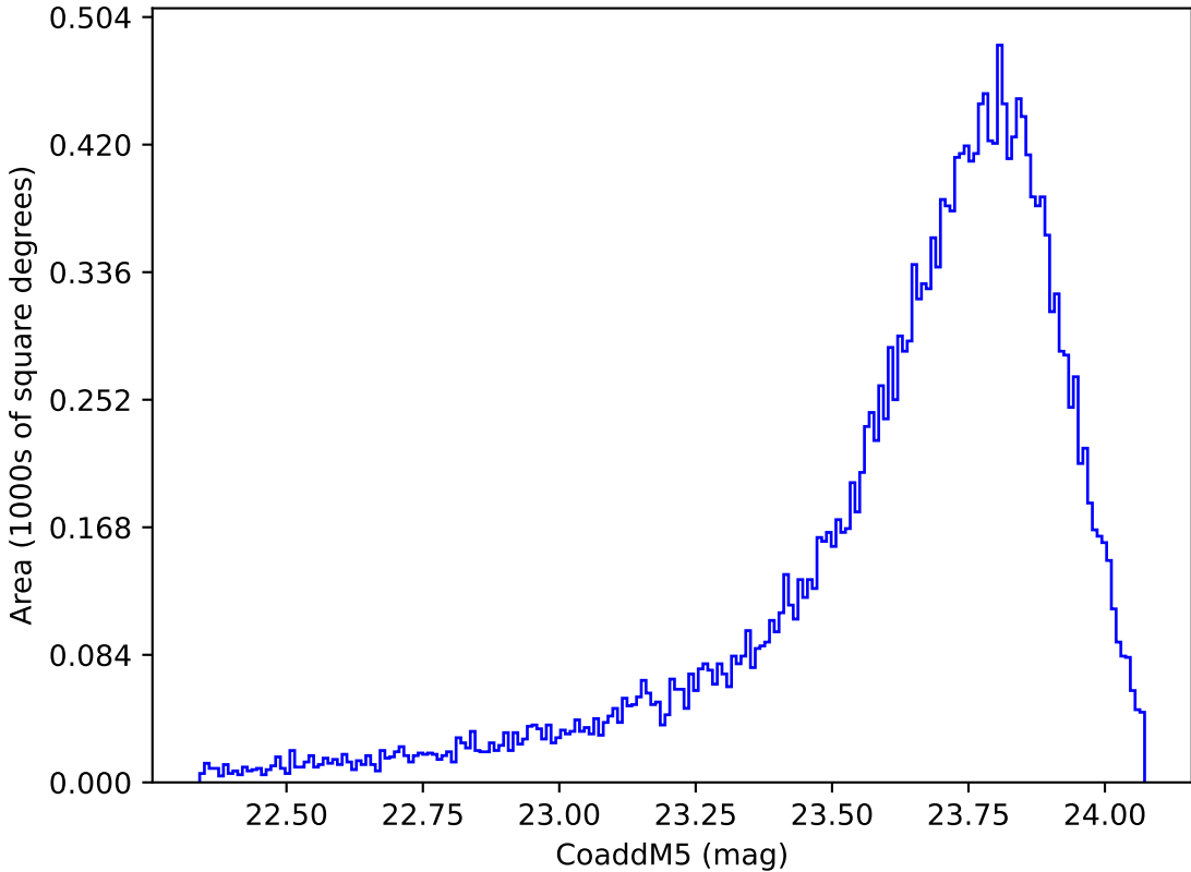
ddf_loaded_half_fl1_v3.4_10yrs Yr 1 y band: CoaddM5
