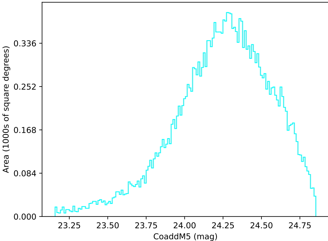
ddf_loaded_half_fl1_v3.4_10yrs Yr 1 u band: CoaddM5
