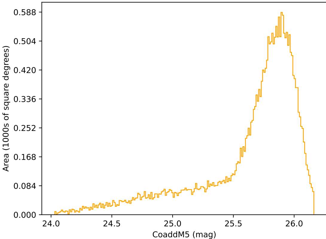
ddf_loaded_half_fl1_v3.4_10yrs Yr 1 r band: CoaddM5
