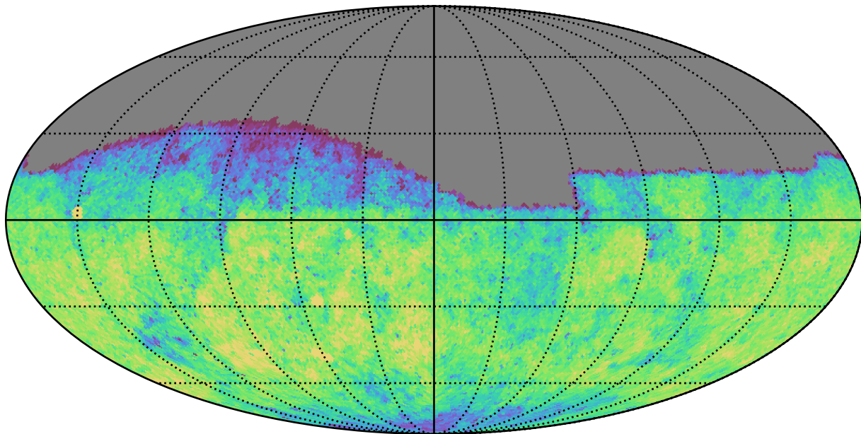
ddf_loaded_half_fl1_v3.4_10yrs Yr 1 g band: CoaddM5
