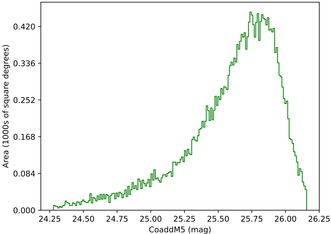
ddf_loaded_half_fl1_v3.4_10yrs Yr 1 g band: CoaddM5
