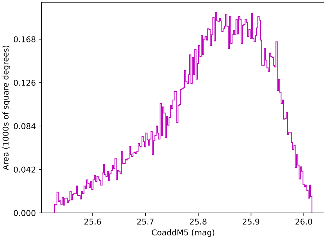
ddf_loaded_half_fl1_v3.4_10yrs WFD z band: CoaddM5
