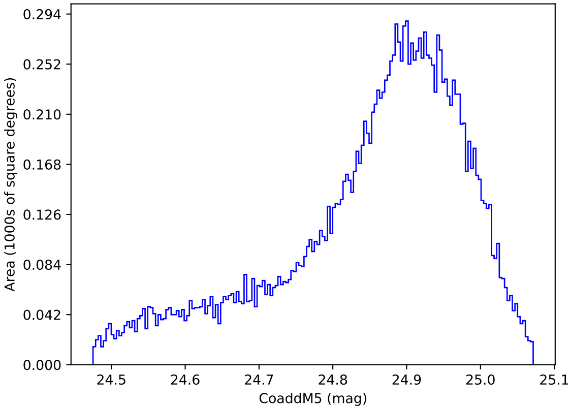
ddf_loaded_half_fl1_v3.4_10yrs WFD y band: CoaddM5
