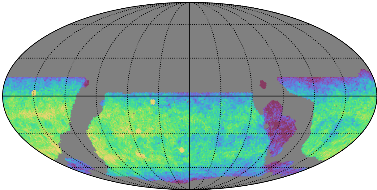
ddf_loaded_half_fl1_v3.4_10yrs WFD u band: CoaddM5
