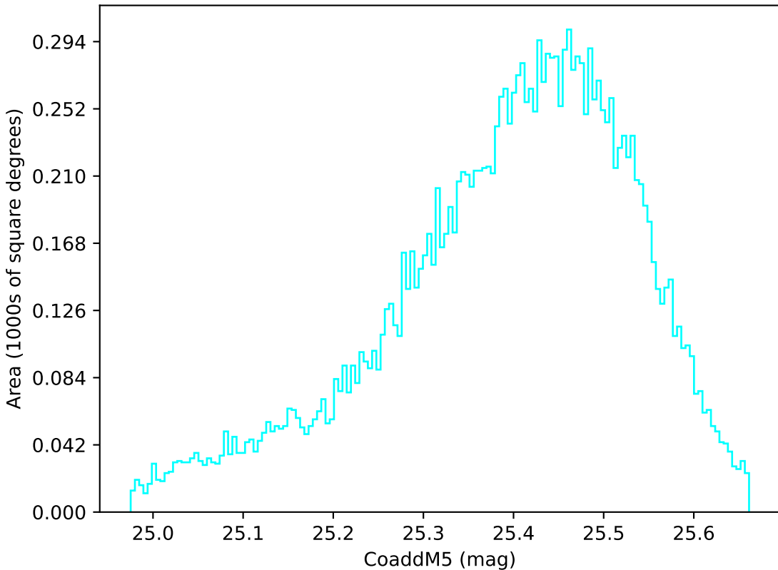
ddf_loaded_half_fl1_v3.4_10yrs WFD u band: CoaddM5
