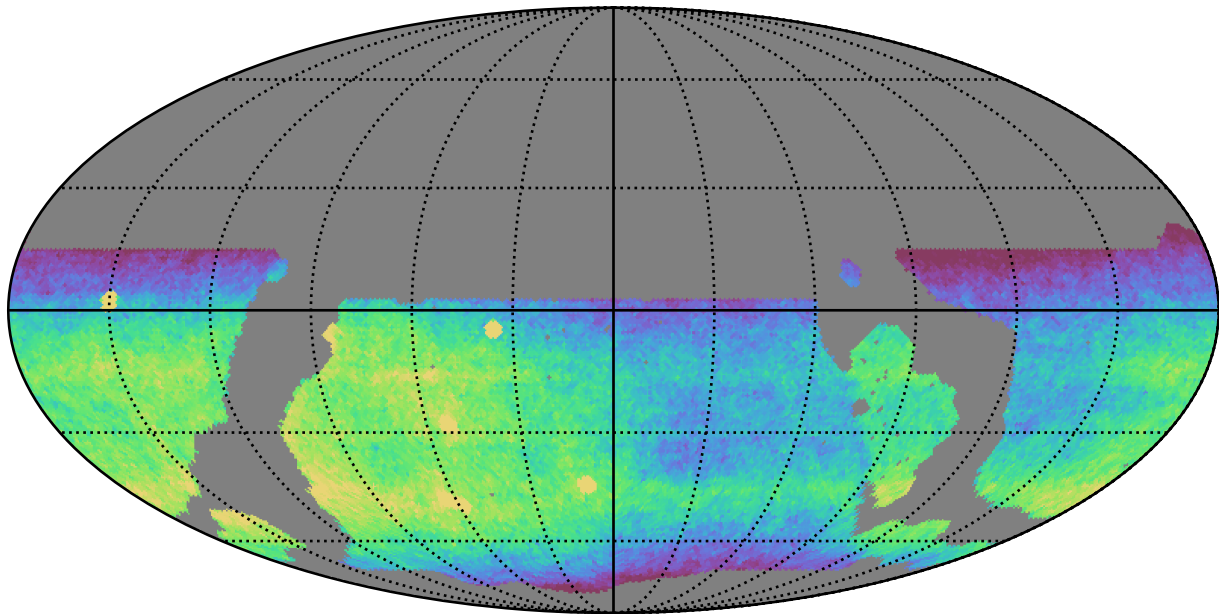
ddf_loaded_half_fl1_v3.4_10yrs WFD r band: CoaddM5
