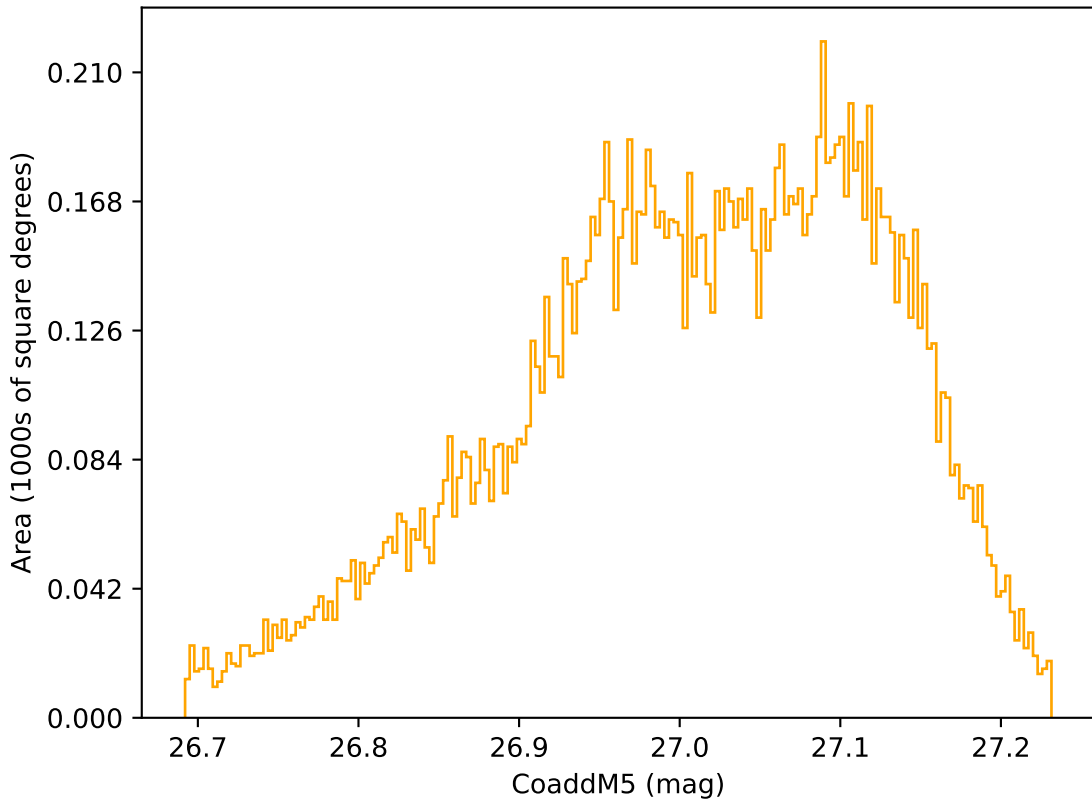
ddf_loaded_half_fl1_v3.4_10yrs WFD r band: CoaddM5
