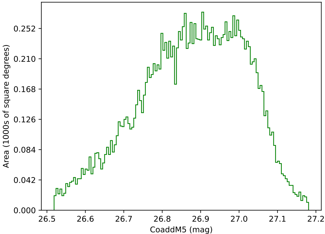
ddf_loaded_half_fl1_v3.4_10yrs WFD g band: CoaddM5
