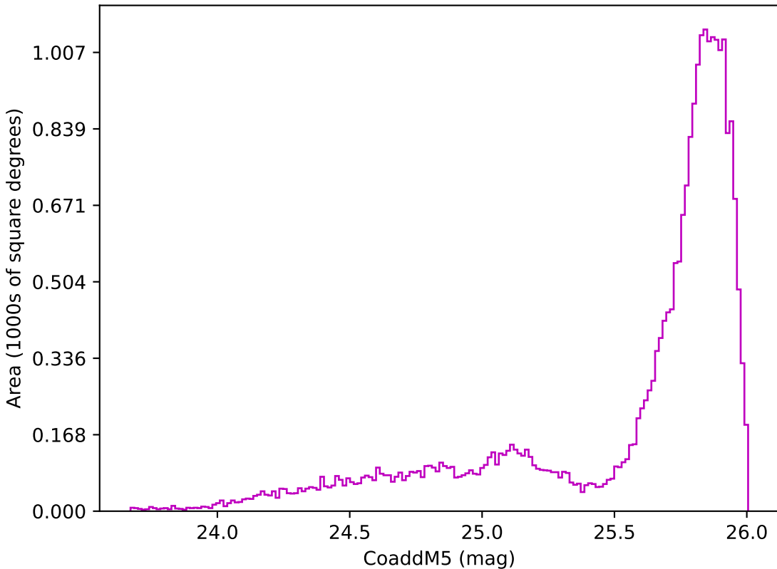
ddf_loaded_half_fl1_v3.4_10yrs All sky z band: CoaddM5
