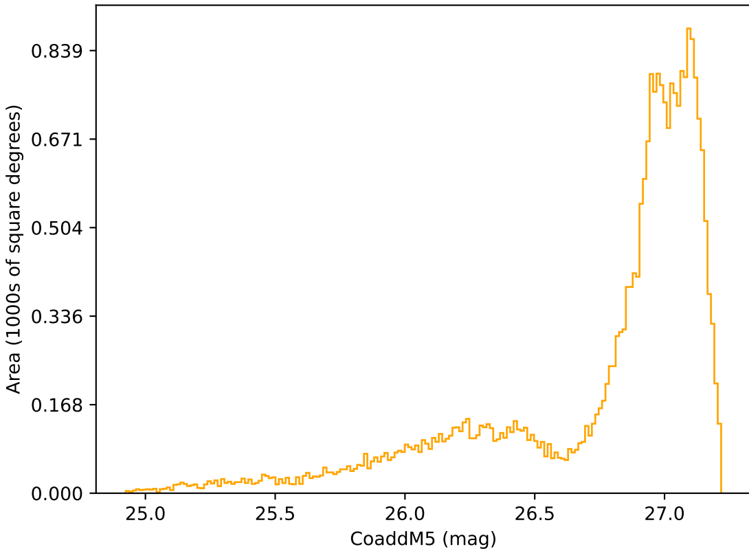
ddf_loaded_half_fl1_v3.4_10yrs All sky r band: CoaddM5
