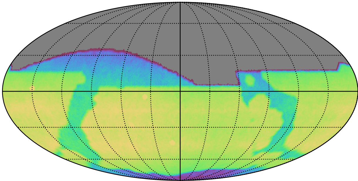
ddf_loaded_half_fl1_v3.4_10yrs All sky i band: CoaddM5
