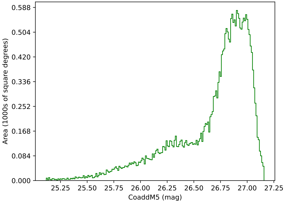
ddf_loaded_half_fl1_v3.4_10yrs All sky g band: CoaddM5
