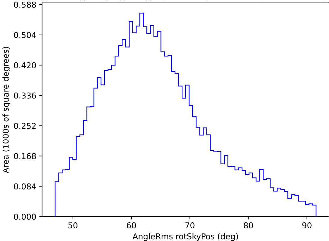
ddf_loaded_half_fl1_v3.4_10yrs WFD y band: AngleRms rotSkyPos
