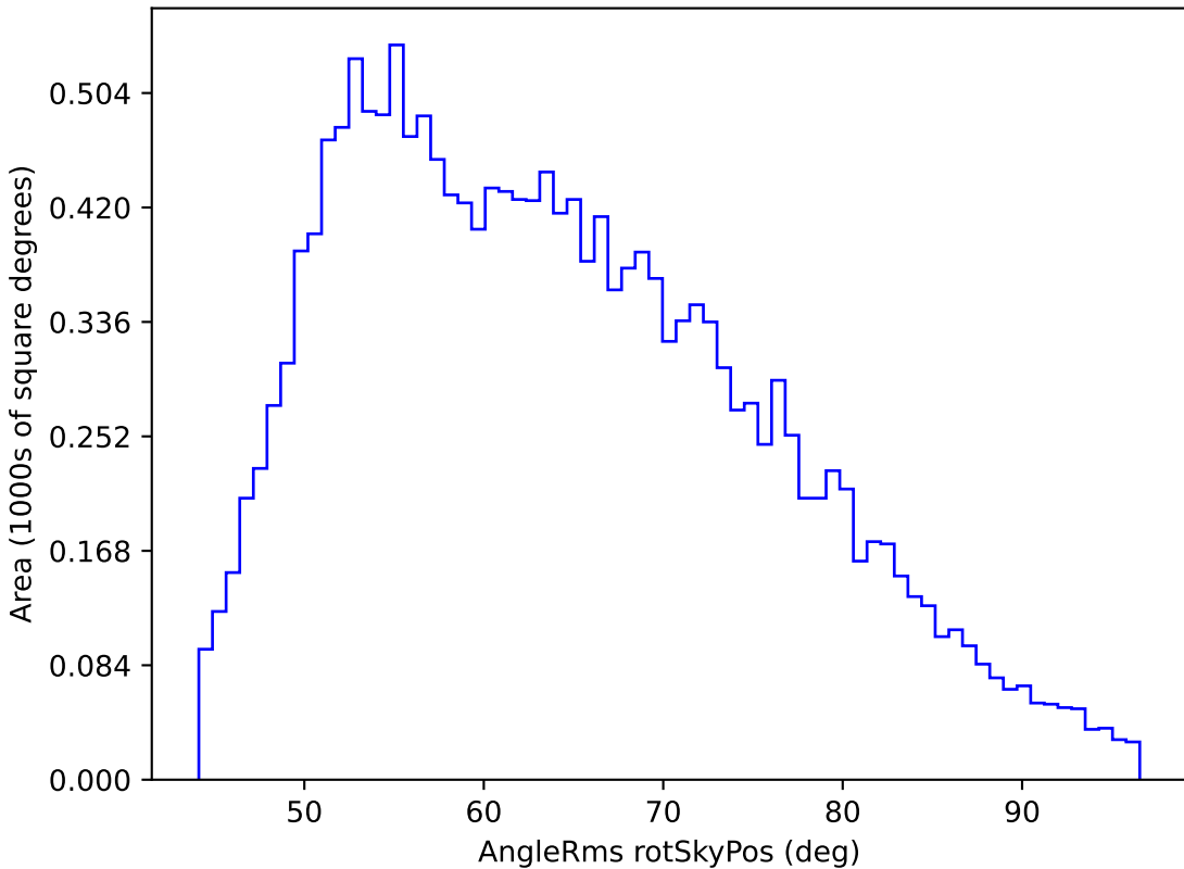
ddf_loaded_half_fl1_v3.4_10yrs WFD u band: AngleRms rotSkyPos
