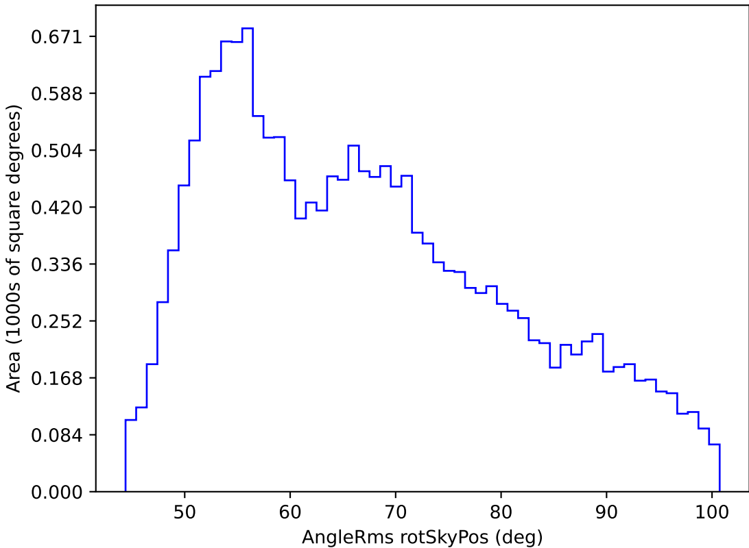
ddf_loaded_half_fl1_v3.4_10yrs WFD g band: AngleRms rotSkyPos
