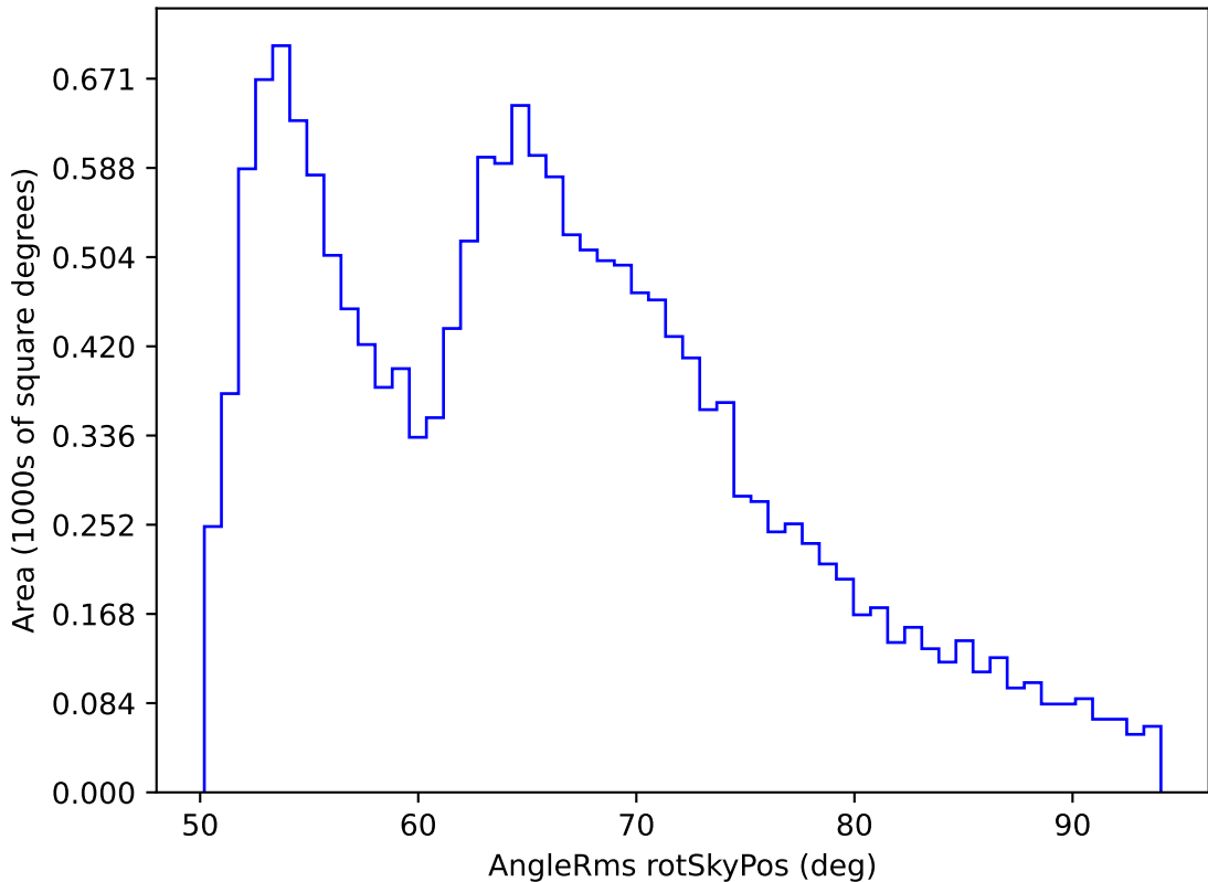
ddf_loaded_half_fl1_v3.4_10yrs WFD all bands: AngleRms rotSkyPos
