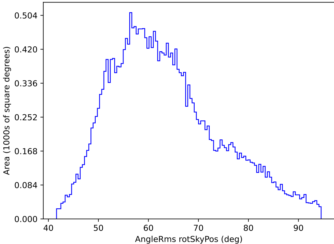
ddf_loaded_half_fl1_v3.4_10yrs All sky z band: AngleRms rotSkyPos
