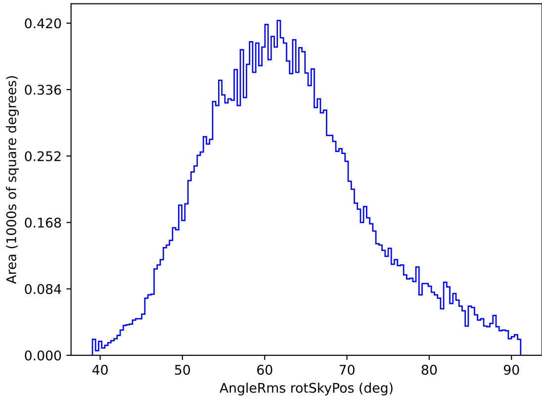
ddf_loaded_half_fl1_v3.4_10yrs All sky y band: AngleRms rotSkyPos
