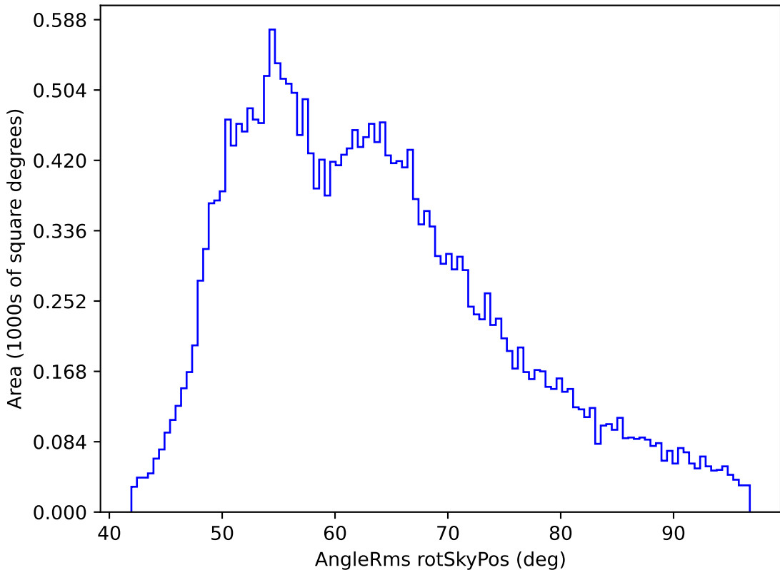
ddf_loaded_half_fl1_v3.4_10yrs All sky r band: AngleRms rotSkyPos
