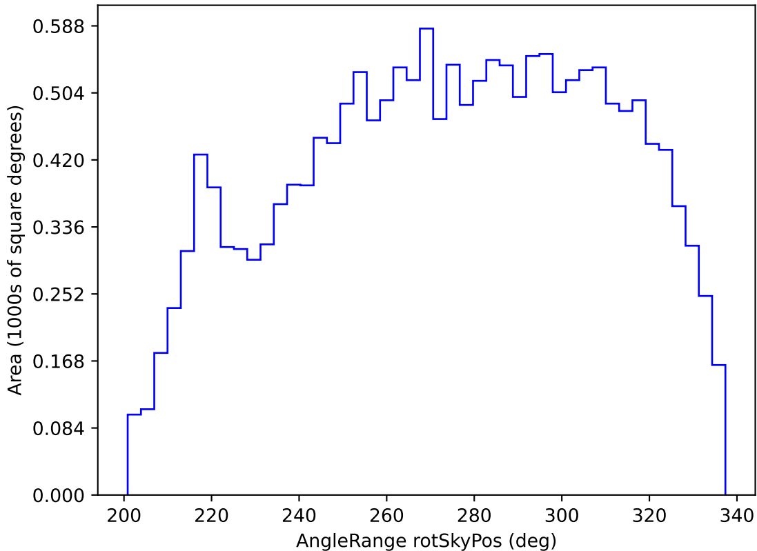
ddf_loaded_half_fl1_v3.4_10yrs WFD y band: AngleRange rotSkyPos
