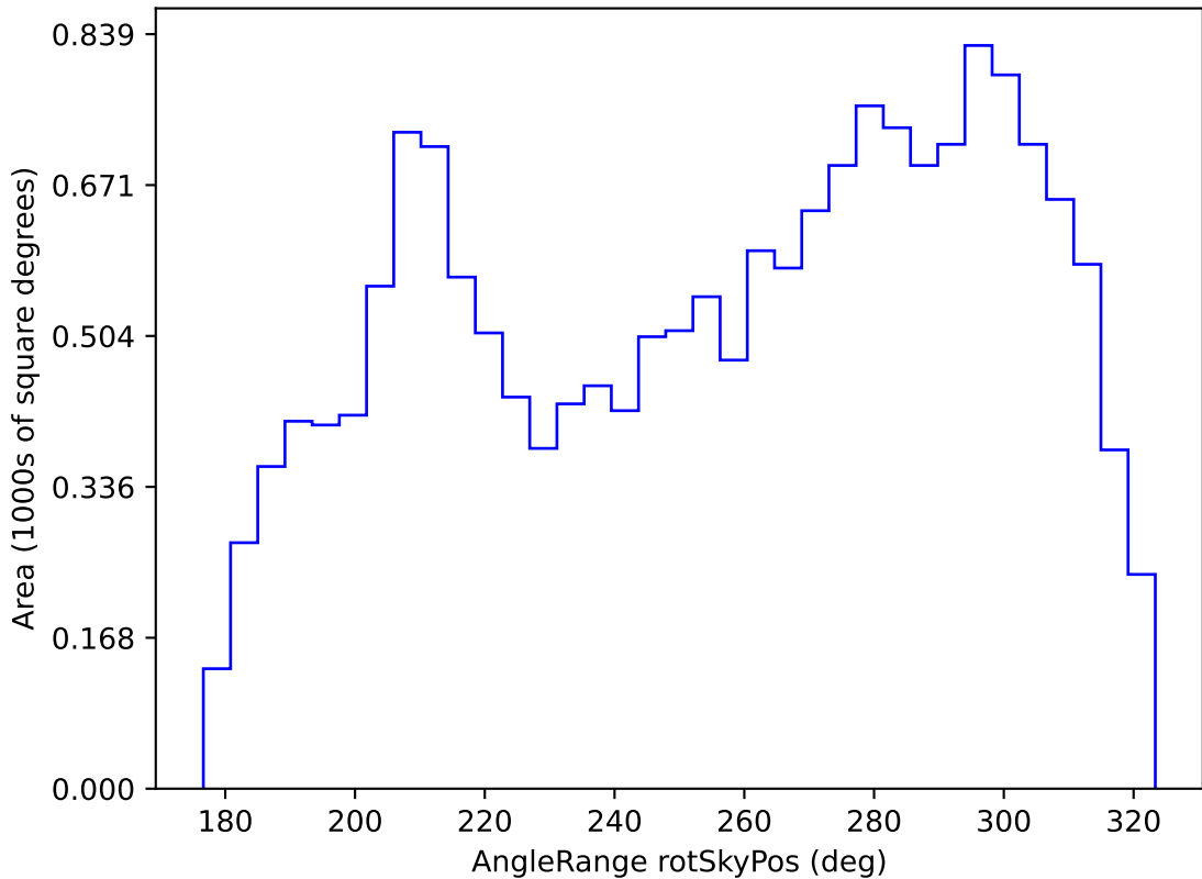
ddf_loaded_half_fl1_v3.4_10yrs WFD u band: AngleRange rotSkyPos
