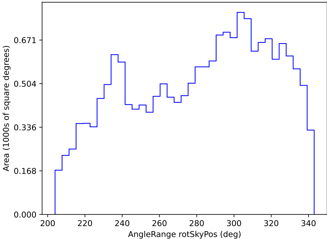
ddf_loaded_half_fl1_v3.4_10yrs WFD r band: AngleRange rotSkyPos
