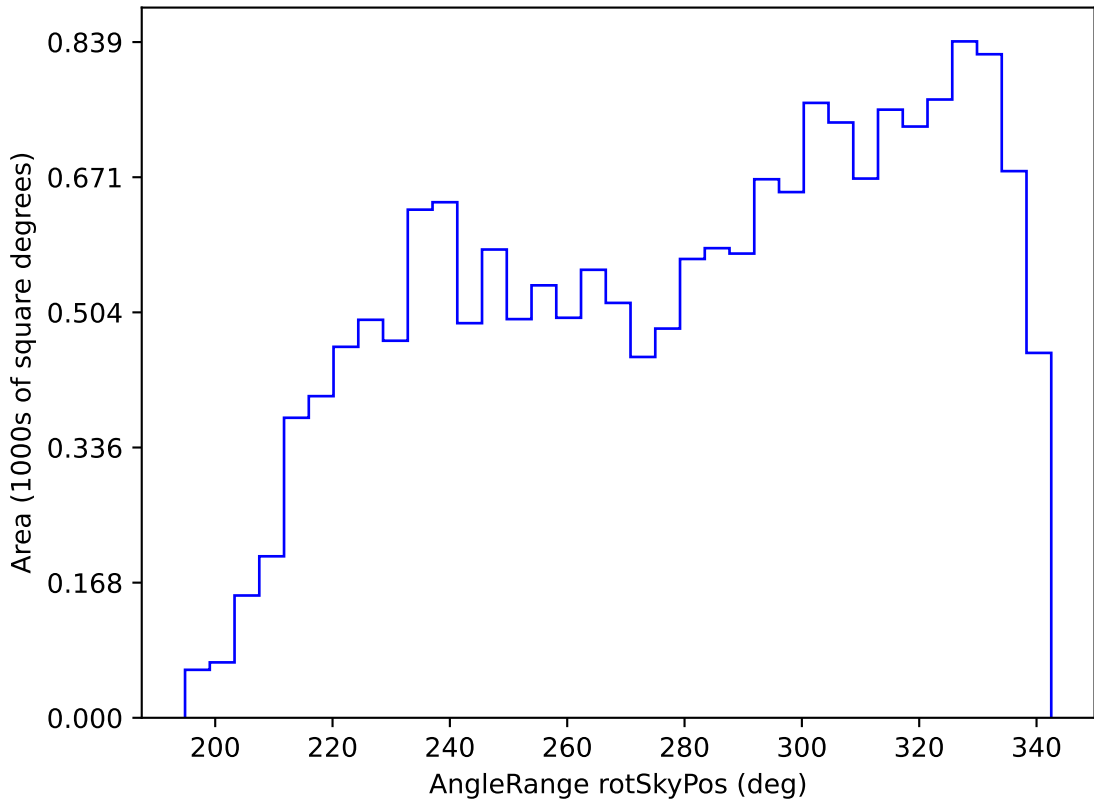
ddf_loaded_half_fl1_v3.4_10yrs WFD i band: AngleRange rotSkyPos
