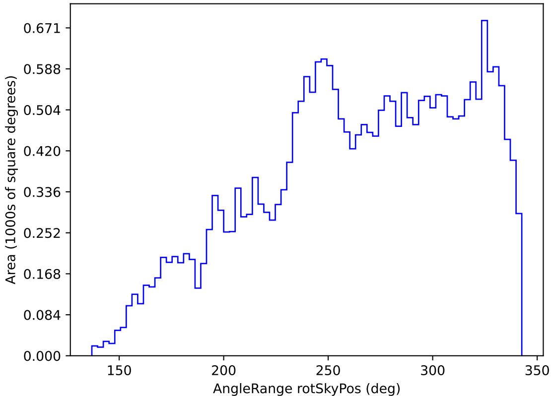
ddf_loaded_half_fl1_v3.4_10yrs All sky z band: AngleRange rotSkyPos
